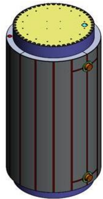
HI-STAR 100MB Dual Function Cask
