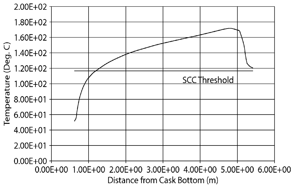
Canister Axial Surface Temperature Profile When Stored in Prior Art VVO of FIG. 1
