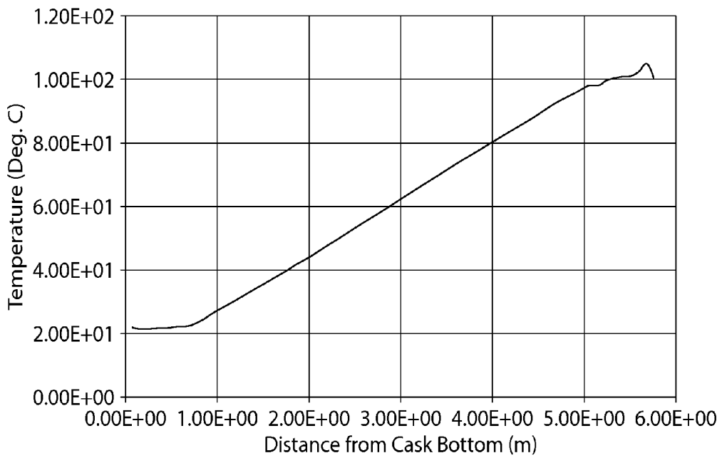
Ventilated Cask Air Temperature Profile Using Prior Art VVO of FIG. 1
