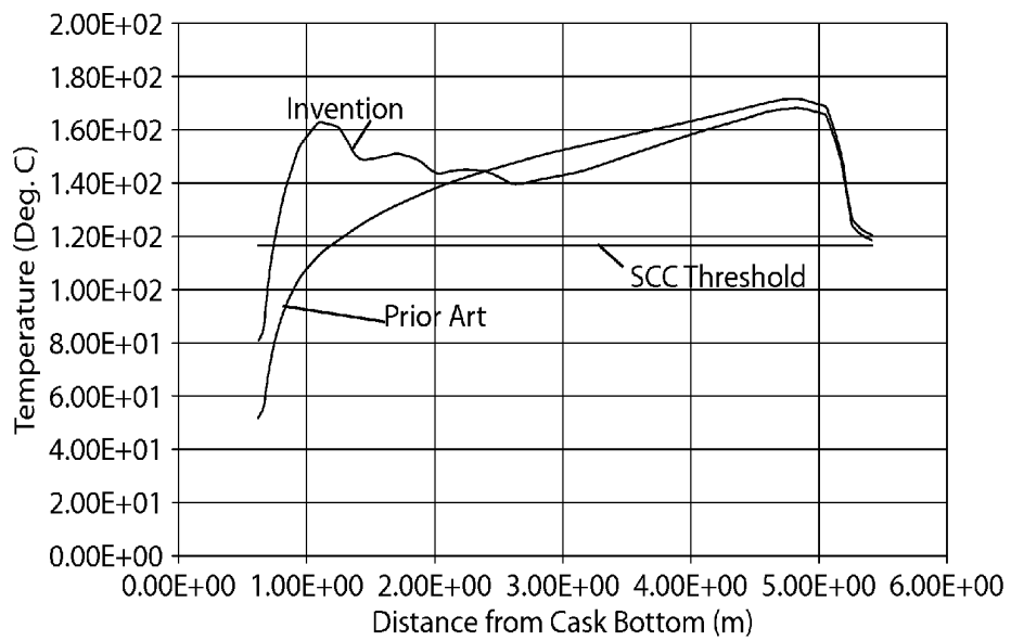
SCC Prone Zone Minimization by Distributed Inlets Design
