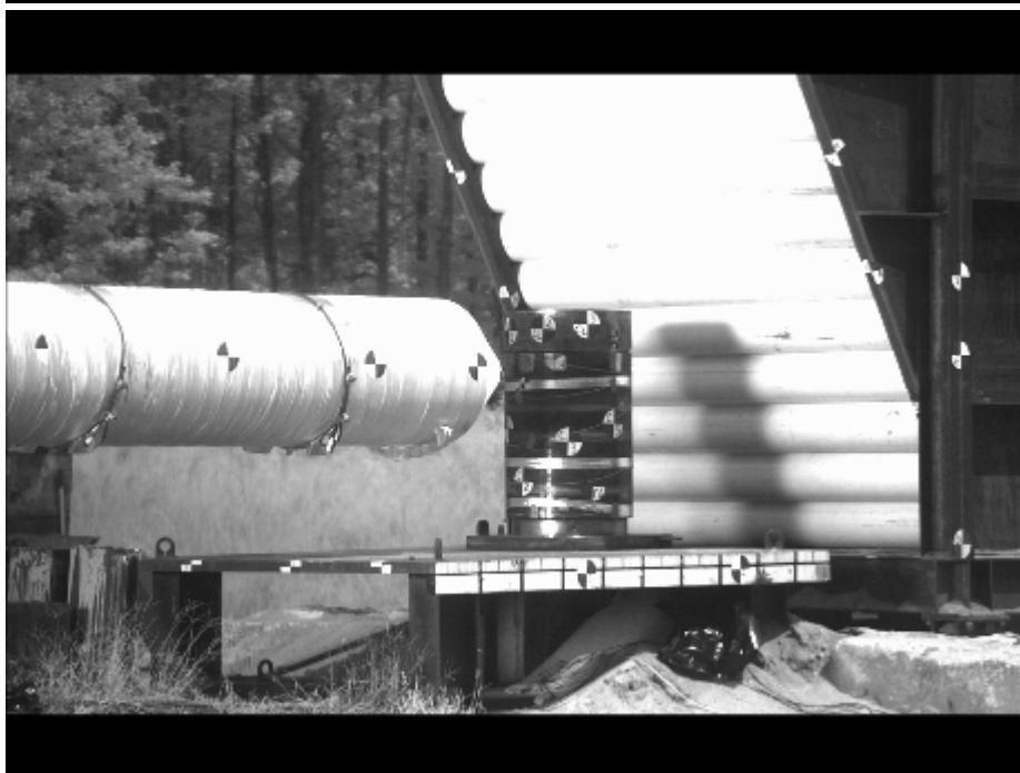
High Speed Photographs of Missile Approaching the Cask at 888 Ft/Sec Just Prior to Impact
